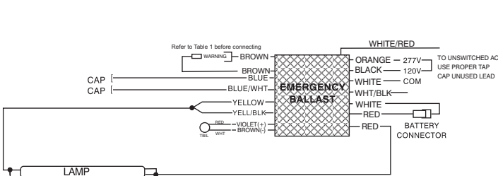
A. ONE (1) LAMP WITHOUT AC BALLAST (14-32W)
