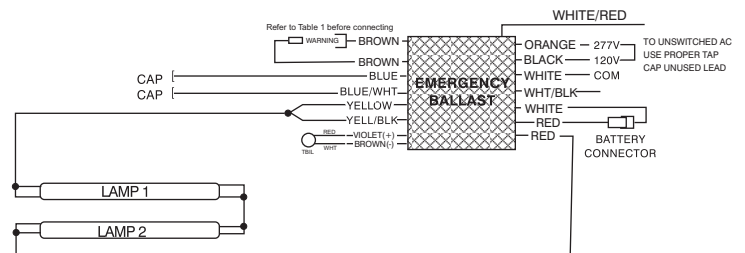
B. TWO (2) LAMP WITHOUT BALLAST (14-32W)
